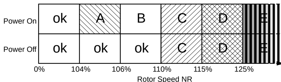
Figure 13-1 Limits for the main rotor RPM (rotor speed, not shown to scale)
